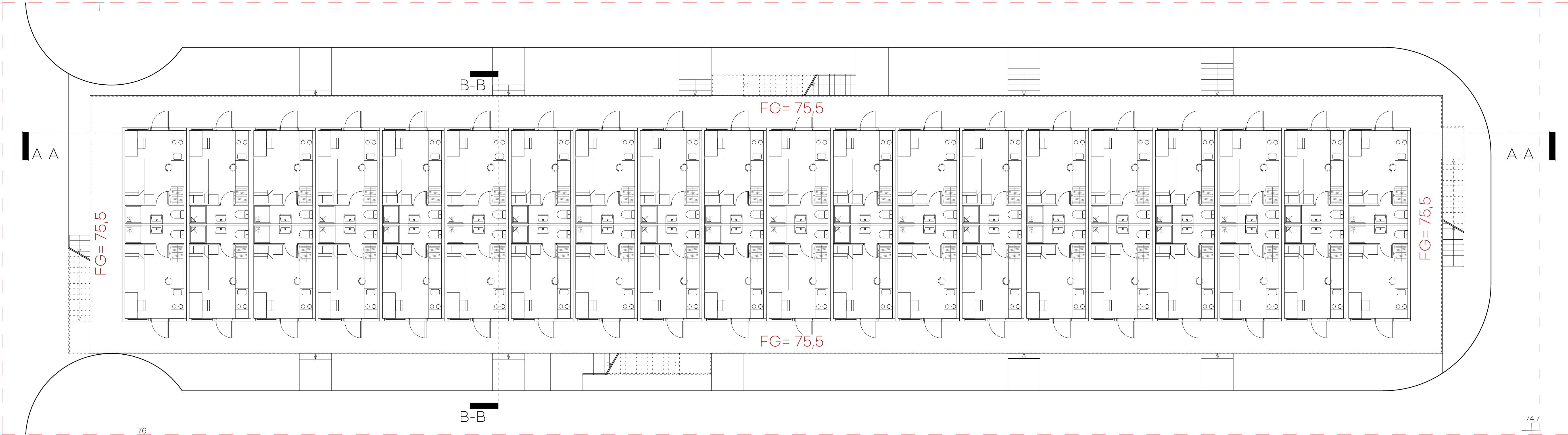
PLANRITNING/ B16 (B15, B17, B18, B19) 1:100
