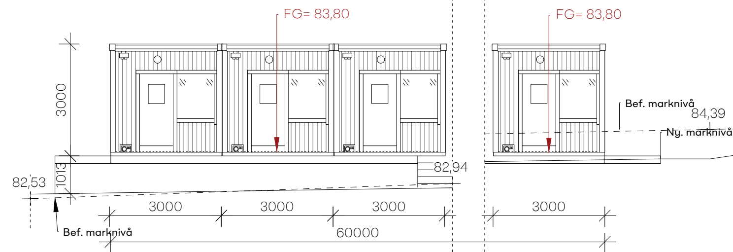
FASAD MOT NORD ÖST/ B3 (B1, B2, B4, B5, B6, B7, B8, B9, B10, B11, B12, B13, B14)
